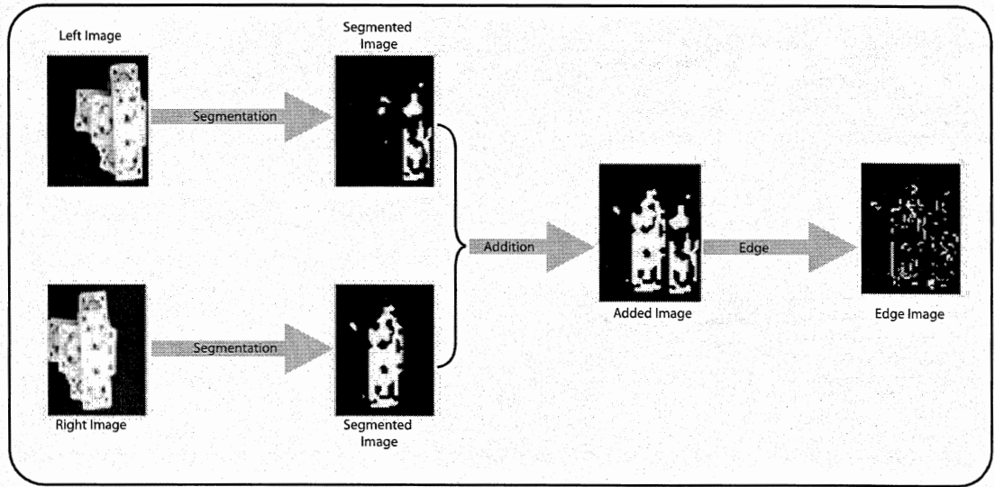
Figure 2. Flow Diagram for Object Feature Extraction.
